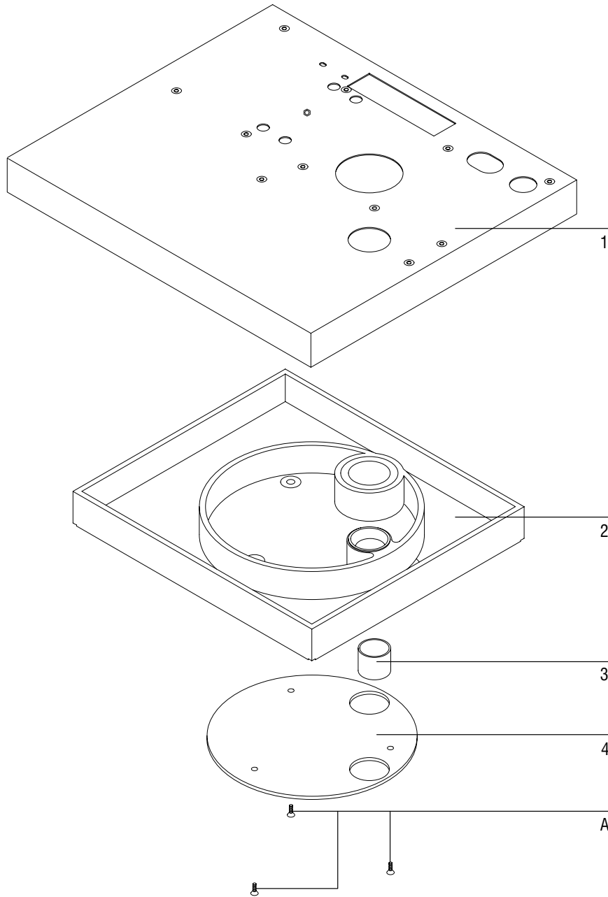
Figure 6-2. Exploding the Oven Top
